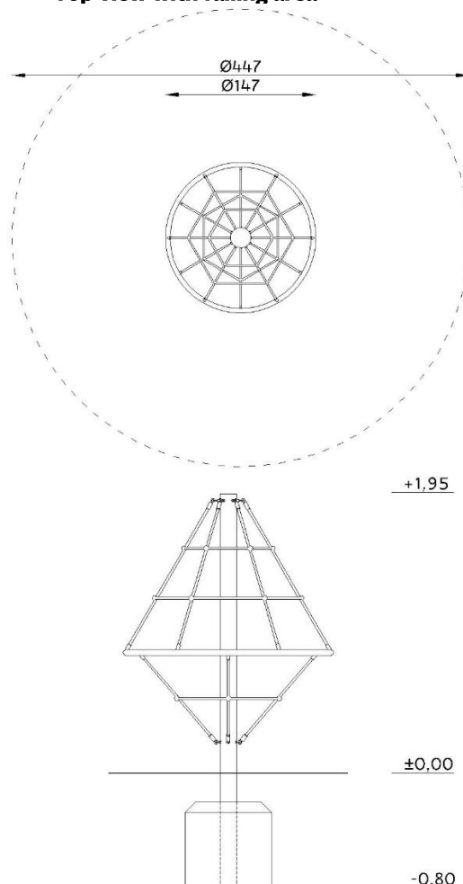
Top view with falling area
